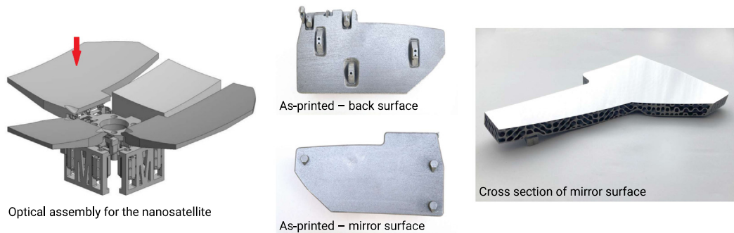
Fig. 45. (left) the nanosatellite optical assembly highlighting the mirror petal; (middle) the as-printed design that underwent XCT acquisition; and (right) a cross section through the reflective surface showing the internal lattice.
